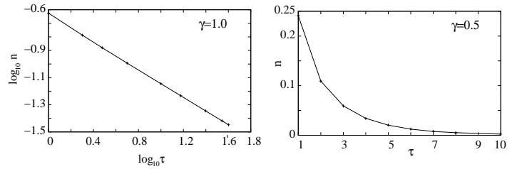
FIG. 2: Numerical integration result for the defect density as a function of \tau for \gamma = 1 and \gamma = 0.5 . The parameter \alpha is chosen such that the system crosses both the gapless phases in the two cases. For \gamma = 1 , we have used log-scale and slope of the straight line is 1/2 indicating a power-law decay of the defect density. For \gamma = 0.5 , we have used linear scale to accentuate the exponential fall of the defect density.
