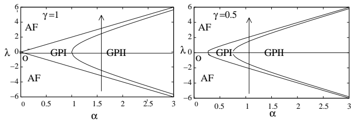
FIG. 1: Phase diagram of the Hamiltonian (5) in the \alpha - \lambda plane for \gamma = 1 and \gamma = 0.5 . Different phases are discussed in the main text. The vertical line shows the direction of quenching.
