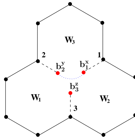
Figure 3. Schematic of the three unpaired b -Majorana fermions formed as a result of cutting the links to the Kitaev spin at the origin. Any two of the three can be given an expectation value (dotted bond).
