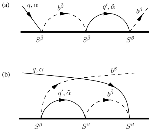
Figure 2. Diagrams contributing to the scaling of Kondo coupling K^\alpha .
