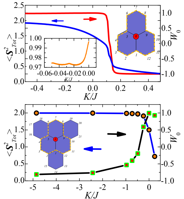
Figure 4. (Color online) (Top) Evolution of expectation values of the flux operator ( W_0 ) and the square of the total spin \mathbf{S}_{Tot} = \mathbf{S} + \sigma_0 at the impurity site with K/J evaluated on a three hexagon fragment. The impurity spin (indicated by the red circle) is coupled to the central spin and the flux is calculated over the boundary. When K = 0 , \langle S_{Tot}^2 \rangle = S(S+1) + \sigma_0(\sigma_0+1) = 3/2 . For K/J \gtrsim 1 , the formation of a bound singlet state means \langle S_{Tot}^2 \rangle \rightarrow 0 . The inset shows the slight decrease of W_0 from 1 for ferromagnetic coupling whereas for antiferromagnetic coupling W_0 changes to -1. (Bottom) W_0 and total spin at the impurity site evaluated for a six hexagon fragment showing the transition to W_0 = -1 state for ferromagnetic coupling. Formation of a bound spin-1 state for K/J \sim -1 is evident from the saturation of \langle S_{Tot}^2 \rangle towards 2. Up to numerical accuracy, it appears that the topological transition and the magnetic transition occur around the same value of K/J .
