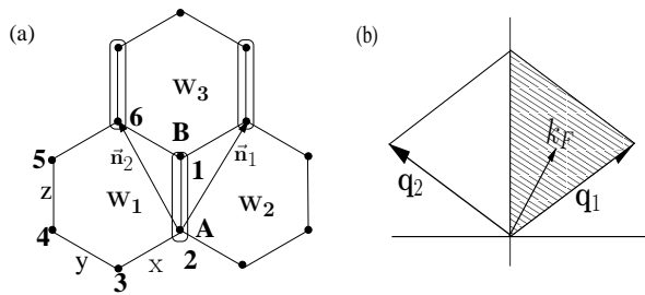
Figure 1. (a) Schematic of a fragment of the Kitaev lattice showing the A and B sites and the x , y and z types of bonds. (b) Figure showing the reciprocal lattice vectors for the A sublattice. The Dirac point for the massless Majorana fermions is denoted by k_F and momentum summations are over the (shaded) half Brillouin zone.
