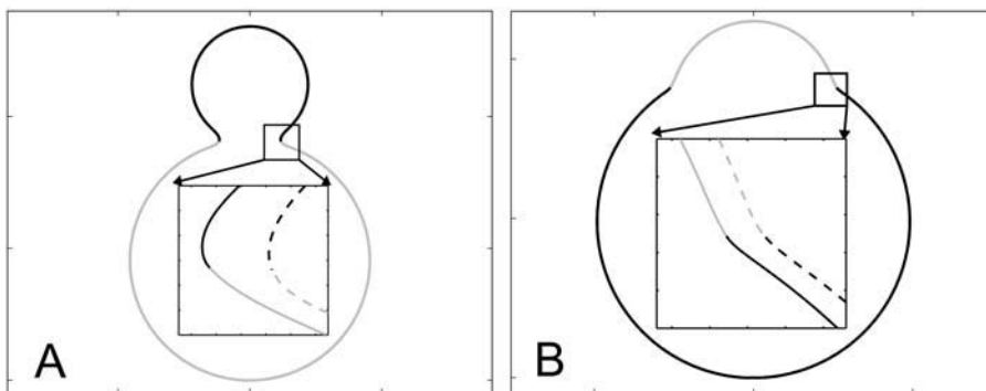
FIGURE 7 Simulated vesicle shapes with area fraction, reduced volume, and boundary radius equal to the experimental vesicles shown in Fig. 2 D ( left ) and Fig. 2 G ( right ). The ratio of mean curvature moduli and dimensionless difference in Gaussian moduli, respectively, were set to \varepsilon = 5 and \hat{\Delta}_g = 3.6 (i.e., the average values found from the analysis of the vesicle shown in Fig. 2 A). Geometrical parameters referring to the simulated shapes are for A: reduced volume v = 0.84 , L_d phase area fraction x_{L_d} = 0.18 , and boundary radius r_b = 0.235 ; and for B: v = 0.98 , x_{L_d} = 0.89 , and r_b = 0.522 . Insets display a comparison of neck geometries for \varepsilon = 5 and \hat{\Delta}_g = 3.6 ( solid lines ) and \varepsilon = 1 and \hat{\Delta}_g = 0 ( dashed lines ).
