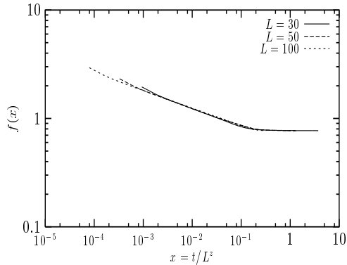
FIG. 3. The scaling function f(x) = L^{z\theta}P(t, L) is plotted against the dimensionless scaled time x = t/L^z for three L -values in d = 3 Glauber Ising model. The observed data collapse has been obtained for z = 2.05 and \theta = 0.166 .
