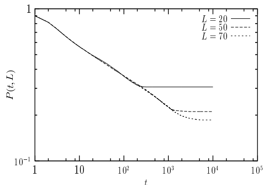
FIG. 5. The persistence probability P(t, L) is plotted against time t (measured as the number of MC steps) for three different lattice sizes L in d = 2 diffusion problem.
