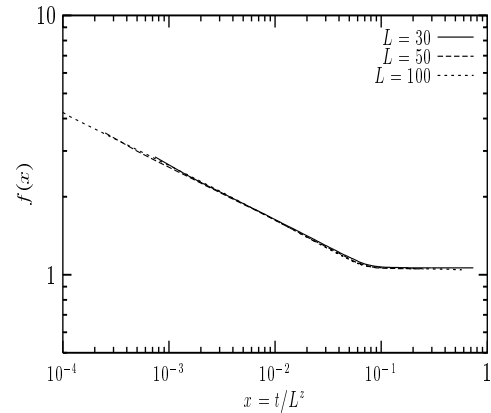
FIG. 2. Same as Fig. 1, except that the scaling function f(x) = L^{z\theta} P(t, L) is plotted against the dimensionless scaling variable x = t/L^z . The data for different L values were found to collapse well to a single curve for \theta = 0.21 and z = 2.12 \pm 0.05 .
