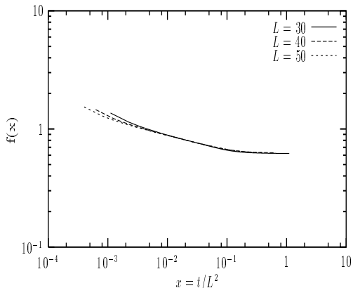
FIG. 4. The figure shows the scaled probability plotted against the dimensionless scaled time in d = 4 Glauber Ising model. We have fixed z = 2 , and find that \theta = 0.12 \pm 0.02 gives the best data collapse.
