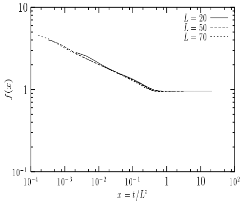
FIG. 6. Same as Fig. 5, except that the scaling function f(x) = L^{z\theta} P(t, L) is plotted against the dimensionless scaling variable x = t/L^z . The data for different L values were found to collapse well to a single curve for \theta = 0.186 and z = 2.05 \pm 0.04 .
