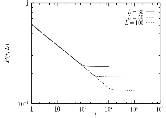
FIG. 1. The persistence probability P(t, L) is plotted against time t (measured in MC steps) for three different lattice sizes L in d = 2 Glauber Ising model.
