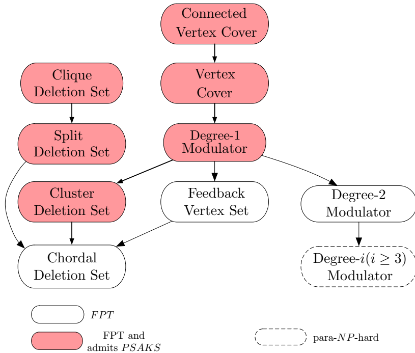
Figure 1: Ecology of Parameters for CONNECTED VERTEX COVER. The parameter values are the minimum possible for a given graph. An arrow from parameter x to parameter y means y \leq x .
