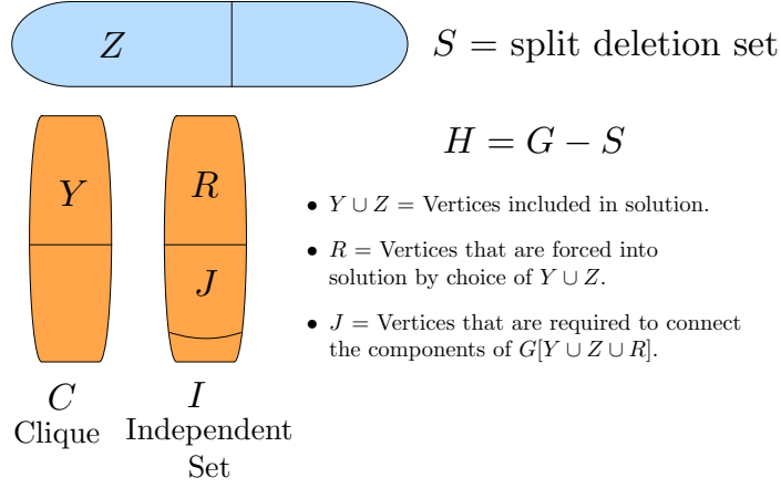
Figure 2: Connected vertex cover parameterized by split deletion set.
