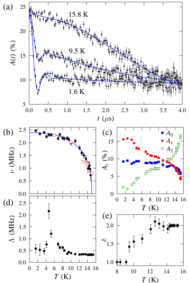
FIG. 2. (color online) Muon spin relaxation results on \alpha - \text{Li}_2\text{IrO}_3 powder. a) Representative zero-field \mu^+ SR spectra measured at several temperatures. Solid lines show fits to the functional form (1) described in the text. b) Extracted temperature dependence of the muon precession frequency \nu (filled circles) fitted to an order parameter behavior (solid line); open squares show the (scaled) order parameter extracted from the intensity of the magnetic Bragg peak observed in neutron powder diffraction data (squares from Fig. 4(inset) in 19 ). c) Temperature dependence of the fitted amplitudes A_0 , A_1 and A_2 . d) The relaxation rate \Lambda and e) the stretching factor \delta .
