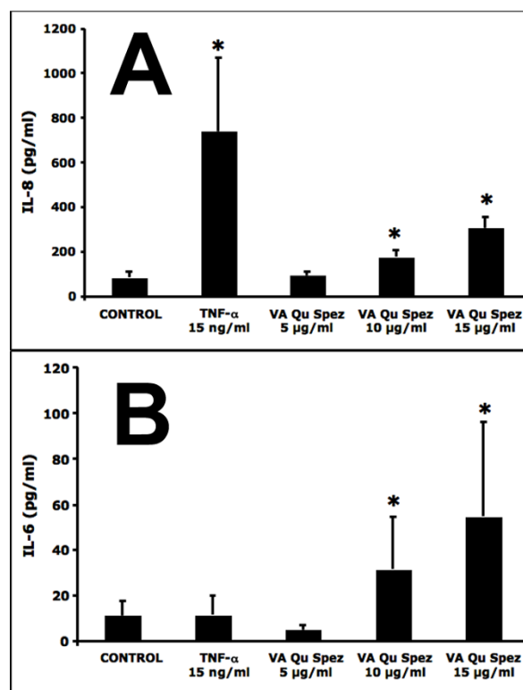
Figure 2 DCs treated with VA Qu Spez show an increased secretion of inflammatory cytokines IL-8 and IL-6. The 4-day-old DCs ( 0.5 \times 10^6 ) were treated with medium alone (Control) or with 15 ng/ml TNF- \alpha or with 5, 10 and 15 \mu g/ml of VA Qu Spez for 48 hours. The secretion (pg/ml) of IL-8 (Panel A) and IL-6 (Panel B) in cell free supernatants were analysed by cytokine bead array assay. Data are presented as mean \pm SEM from five to six independent donors. Statistical significance (*, p < 0.05 ) as analysed by Mann-Whitney test is indicated.
