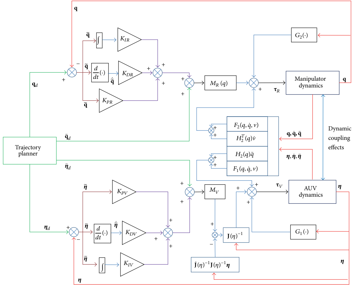
FIGURE 3: Block diagram of model reference control.
