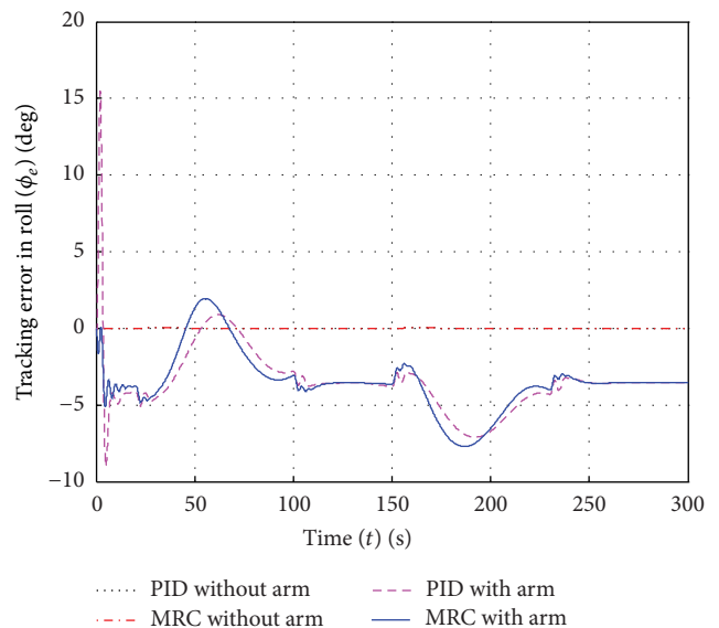
FIGURE 9: Tracking errors in roll for a given 3D trajectory.
