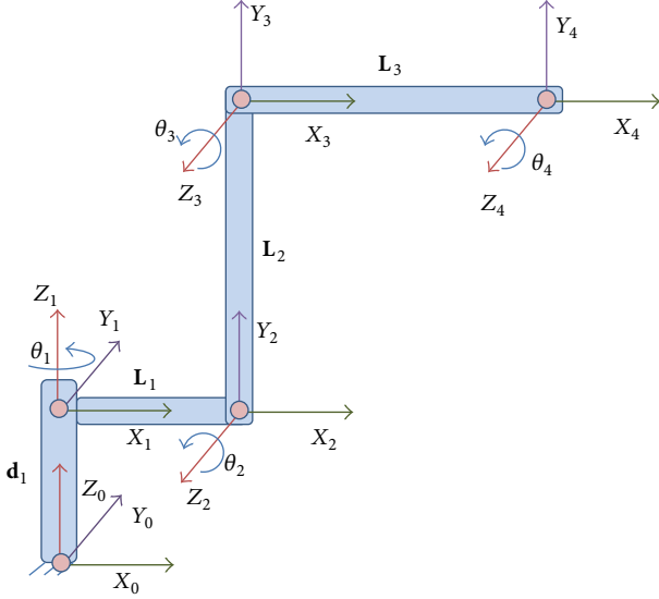
FIGURE 2: Establishing link coordinate systems of the manipulator.
