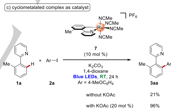
Scheme 5. Key mechanistic studies.
