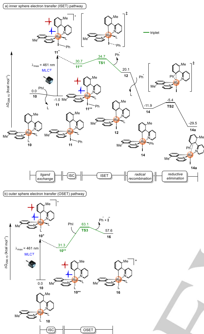
Figure 4. Relative Gibbs free energy profile in kcal mol -1 with respect to 10 at the PBE0-D3(BJ)/6-311++G(d,p),def2-TZVP(Ru,I),SDD(Ru,I)+SMD(1,4dioxane)//B3LYP-D3(BJ)/6-31G(d),def2-SVP(Ru,I),SDD(Ru,I) level of theory for photo-induced ruthenium-catalyzed C–H arylation via a) inner-sphere electron transfer (ISET) and b) outer-sphere electron transfer (OSET) pathways. L = AcOH.
