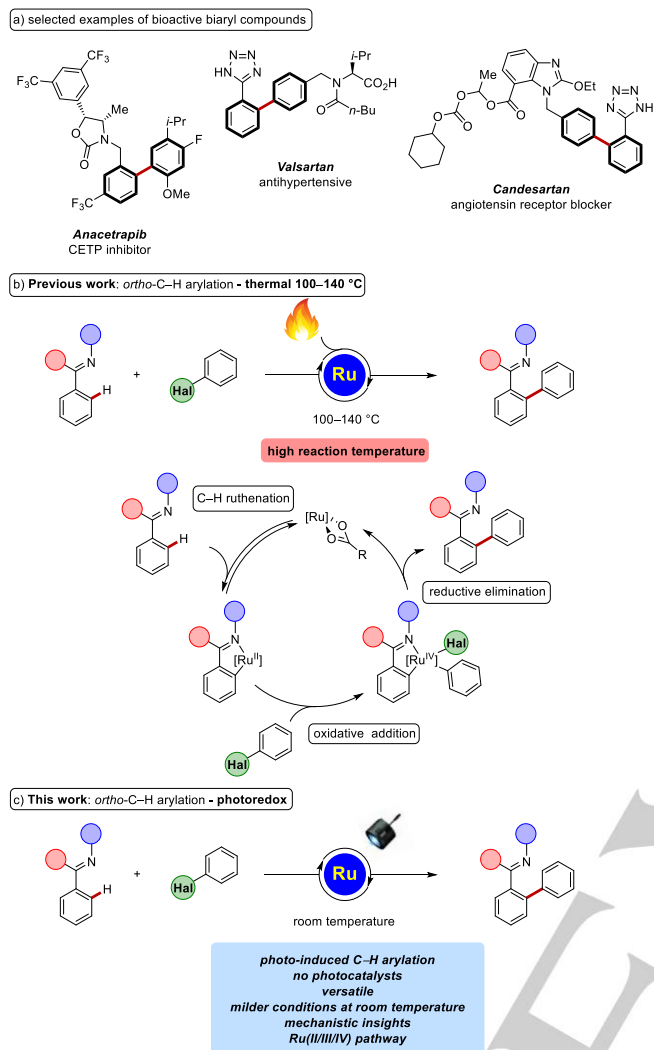
Figure 1. (a) Bioactive biaryls and ruthenium-catalyzed C–H arylations; (b) under thermal reaction condition and (c) under photoredox condition.
