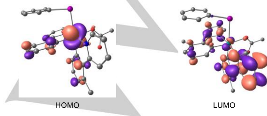
b) HOMO and LUMO of ruthenacycle 11
