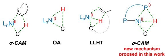
(b) Mechanistic studies in this work
