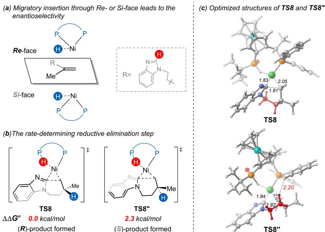
Fig. 11 (a) Migratory insertion by the Re- or Si-face of the substrate; (b) the two competing reductive elimination transition states; (c) the optimized structures of TS8 and TS8* with selected bond distances in Å.
