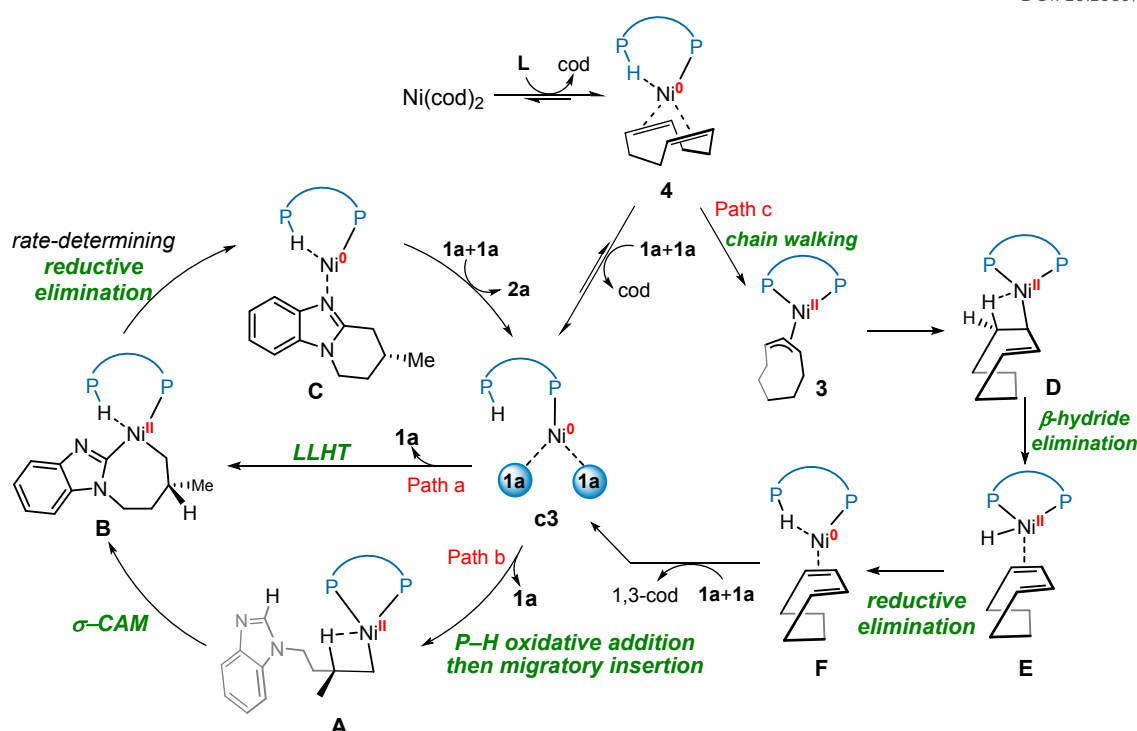
Scheme 4 Overall mechanism of the nickel-catalyzed hydroarylation.
