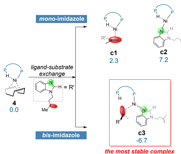
Fig. 4 The possible ligand-substrate exchanges and representative substrate-coordinated complexes with energies in kcal/mol.
