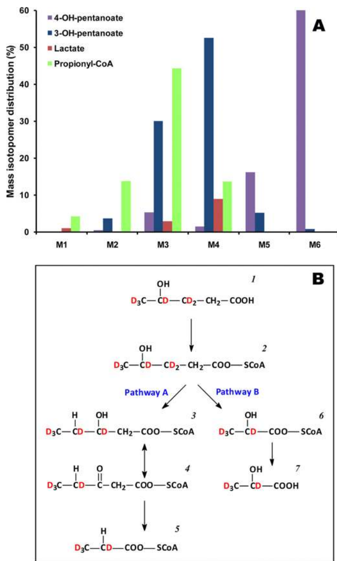
FIGURE 9. Identification of the metabolites of 4-hydroxypentanoate by mass isotopomer analysis. A, mass isotopomer distribution of synthetic 4-hydroxy-[3,3,4,5,5,5- ^2\text{H}_6 ]pentanoate and its metabolites assayed in liver perfusate (3-hydroxypentanoate, lactate) and in liver tissue (propionyl-CoA). B, scheme of the metabolism of M6 4-hydroxy-[3,3,4,5,5,5- ^2\text{H}_6 ]pentanoate in liver. ^2\text{H} atoms are designated as D. The compounds shown are: 4-hydroxypentanoate M6 (compound 1), 4-hydroxypentanoyl-CoA M6 (compound 2), 3-hydroxypentanoyl-CoA M5 (compound 3), released as the free acid, 3-ketopentanoyl-CoA M4 (compound 4), propionyl-CoA M4 (compound 5), lactyl-CoA M4 (compound 6), and lactate M4 (compound 7).
