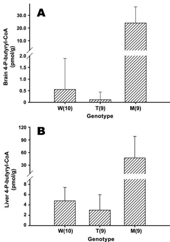
FIGURE 11. A and B, concentrations of 4-phosphobutyryl-CoA in the brains (A) and liver (B) of wild-type (W), heterozygote (T), and mutant (M) mice deficient in succinic semialdehyde dehydrogenase.
