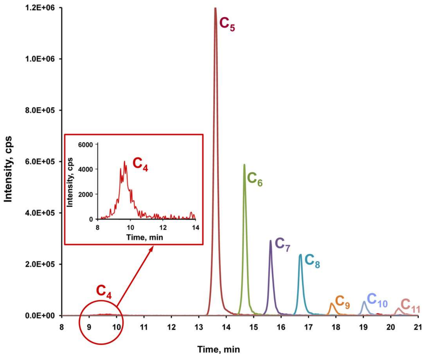
FIGURE 2. Retention times and relative abundances of 4-phosphoacyl-CoAs assayed under identical LC-MS/MS conditions in extracts of rat livers perfused with 2 mM of C 4 to C 11 4-hydroxy- n -acids (composite chromatogram).
