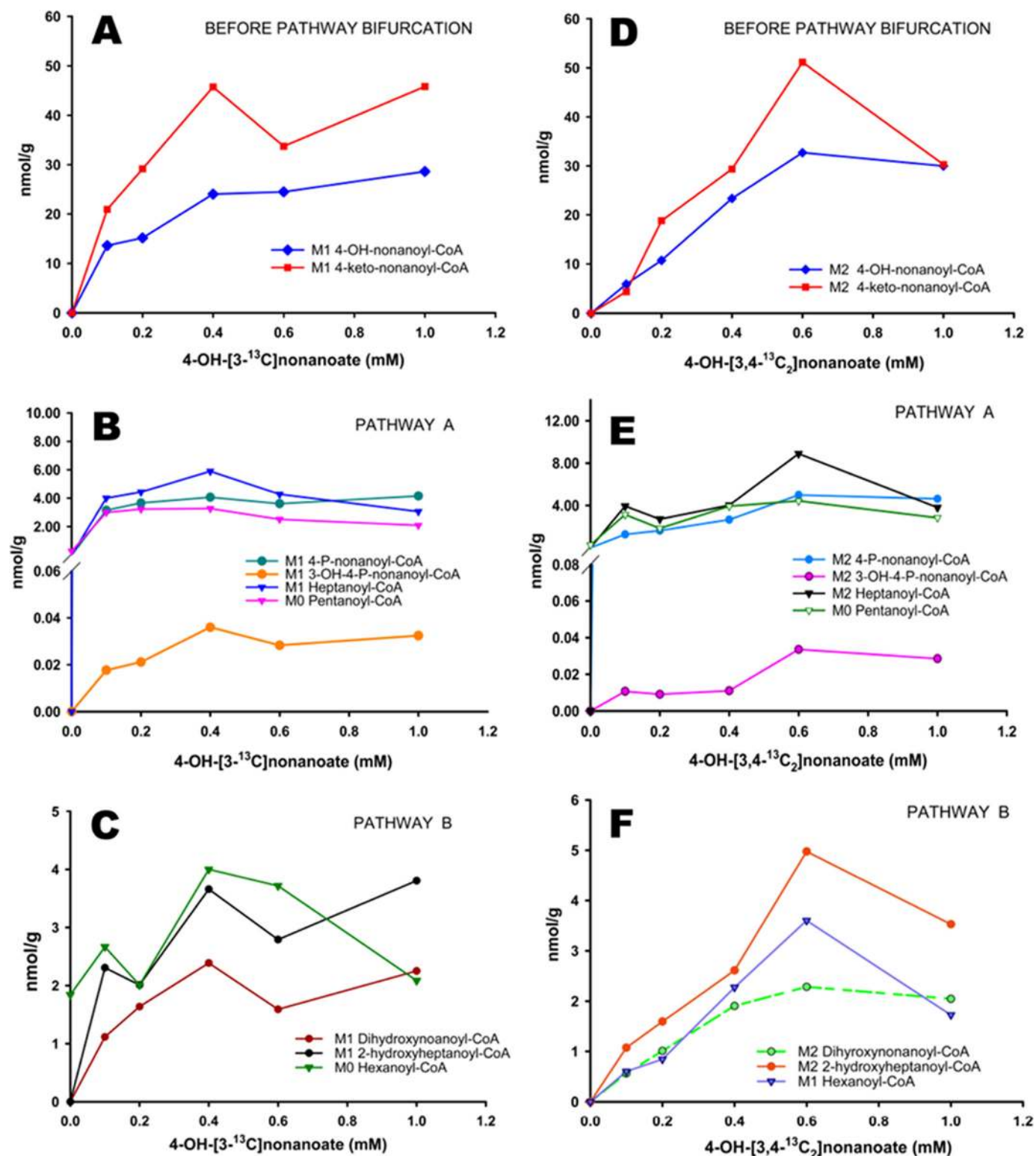
FIGURE 7. Accumulation of acyl-CoAs in livers perfused with increasing concentrations of 4-hydroxy-[3- 13 C]nonanoate (A-C) and 4-hydroxy-[3,4- 13 C 2 ]nonanoate (D-F). Unlabeled, singly labeled, and doubly labeled compounds are designated as M, M1, and M2. The three levels of panels group acyl-CoAs formed (i) before the bifurcation of the pathways outlined in Fig. 4 (A and D), (ii) in pathway A (B and E), and (iii) in pathway B (C and F).
