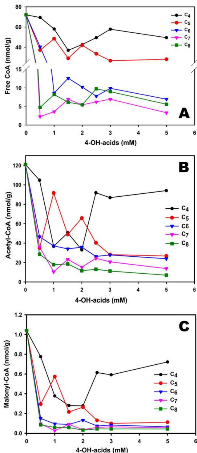
FIGURE 10. Evidence for CoA trapping in livers perfused with increasing concentrations of 4-hydroxyacids with 4–8 carbons. Concentrations of free CoA (A), acetyl-CoA (B), and malonyl-CoA (C) are shown.
