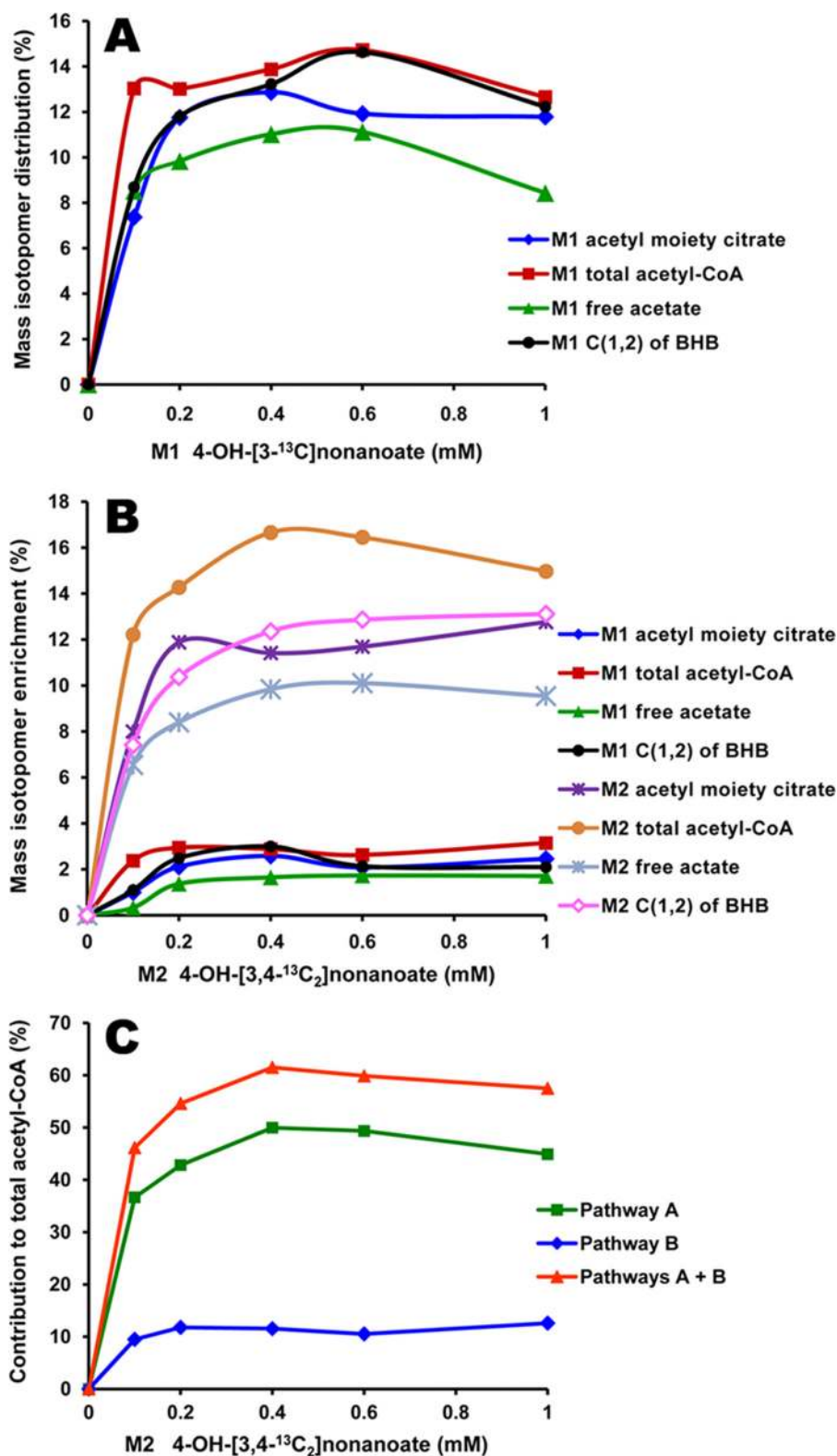
FIGURE 8. Labeling of acetyl-CoA and its proxies. A and B , labeling of acetyl-CoA and its proxies in livers perfused with increasing concentrations of 4-hydroxy-[3- 13 C]nonanoate ( A ) or 4-hydroxy-[3,4- 13 C 2 ]nonanoate ( B ). The acetyl-CoA proxies are the acetyl moiety of citrate, free acetate, and C-1+2 of BHB. C , contribution of 4-hydroxy-[3,4- 13 C 2 ]nonanoate to liver acetyl-CoA via pathway A of Fig. 4 ( middle curve ) and via pathway B of Fig. 4 ( lower curve ). The upper curve is the total contribution of the substrate to acetyl-CoA.
