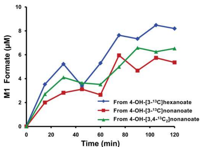
FIGURE 5. Release of [ 13 C]formate by livers perfused with recirculating buffer containing 2 mM 4-OH-[3- 13 C]nonanoate (■), 4-OH-[3,4- 13 C 2 ]nonanoate (▲), or 4-OH-[3- 13 C]hexanoate (◆). The three profiles are not statistically different.
