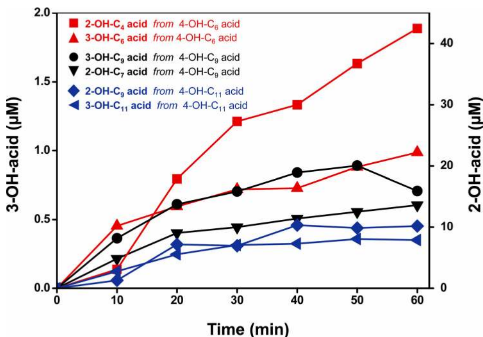
FIGURE 3. Conversion of C 6 , C 9 and C 11 4-hydroxyacids to (i) 3-hydroxyacids with the same number of carbons and (ii) 2-hydroxyacids with two carbons less than the original substrate. Each color corresponds to the two products of a given 4-hydroxyacid. Not shown on the figure are the accumulations of free carboxylic acids with two and three carbons less than the original substrate.
