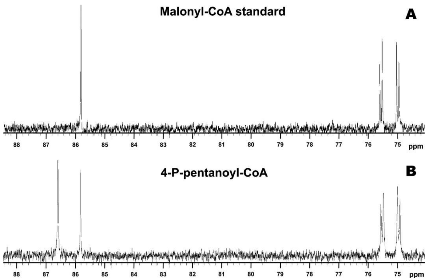
FIGURE 1. ^{31}\text{P} -NMR of a malonyl-CoA standard (A) and of 4-phosphopentanoyl-CoA isolated from a rat liver perfused with 4-hydroxypentanoate (B). Note the additional peak at the chemical shift value of 86.615 in the spectrum of 4-phosphopentanoyl-CoA.
