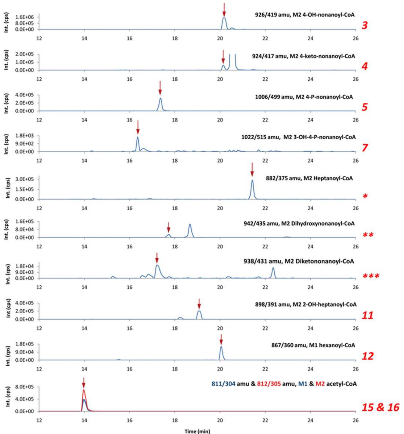
FIGURE 6. Identification of singly labeled (M1) and doubly labeled (M2) acyl-CoAs in a liver perfused with 2 mM doubly labeled 4-OH-[3,4- ^{13}\text{C}_2 ]nonanoate. The vertical scale of each strip refers to the intensity of the signal expressed in counts per second. Numbers in red italics to the right of the strips refer to intermediates shown in Fig. 4. *, M2 heptanoyl-CoA is an intermediate of one of the \beta -oxidation cycles between compounds 9 and 14 (Fig. 4). **, M2 dihydroxynonanoyl-CoA is an intermediate of the \beta -oxidation cycle between compounds 3 and 11 (Fig. 4). ***, M2 diketnonanoyl-CoA is an intermediate of the \beta -oxidation of compound 4 to compound 11, without passing by compound 3 (Fig. 4). amu , atomic mass units.
