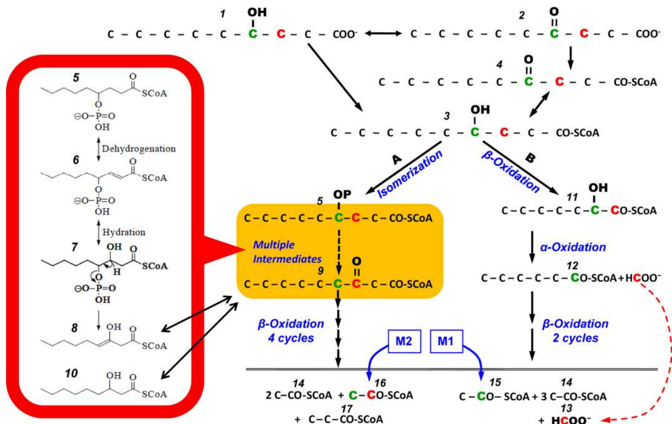
FIGURE 4. Proposed scheme of the catabolism of 4-hydroxyacids using 4-hydroxynonanoate as an example. Carbons 3 and 4 of the substrate are colored in red and green, respectively, to facilitate the tracing of their fates through pathways A and B. Note that the doubly labeled substrate forms acetyl-CoA, part of which is doubly labeled (M2) via pathway A and singly labeled (M1) via pathway B. Formate, derived from carbon 3 of the substrate, is formed via pathway B. The compounds shown are 4-hydroxynonanoate (compound 1), 4-ketononanoate (compound 2), 4-hydroxynonanoyl-CoA (compound 3), 4-ketononanoyl-CoA (compound 4), 4-phosphononanoyl-CoA (compound 5), 4-phospho-2-ene-nonanoyl-CoA (compound 6), 3-hydroxy-4-phosphononanoyl-CoA (compound 7), enol form of 3-ketononanoyl-CoA (compound 8), 3-ketononanoyl-CoA (compound 9), 3-hydroxynonanoyl-CoA (compound 10), 2-hydroxyheptanoyl-CoA (compound 11), hexanoyl-CoA (compound 12), formate (compound 13), unlabeled acetyl-CoA (compound 14), singly labeled (M1) acetyl-CoA (compound 15), doubly labeled (M2) acetyl-CoA (compound 16), and propionyl-CoA (compound 17). Note that for even-chain 4-hydroxyacids with at least six carbons, pathway A leads to acetyl-CoA, whereas pathway B leads to acetyl-CoA, propionyl-CoA, and formate.
