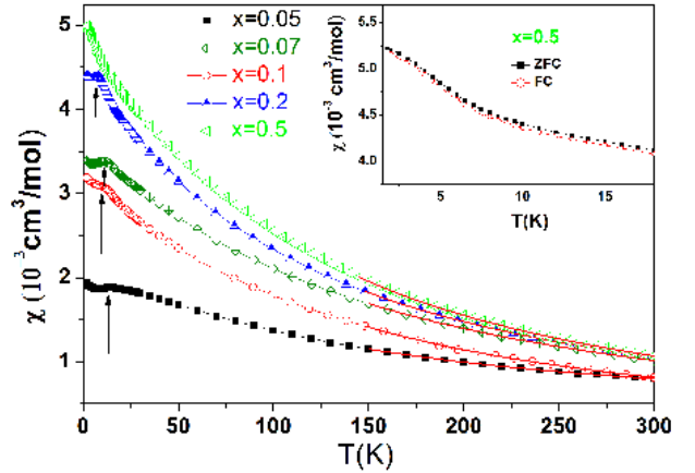
FIG. 4: (Color online) Magnetic susceptibility \chi(T) vs T for x = 0.05 to 0.2 and x=0.5 . The red line indicates fitting by CW behavior \chi = \chi_0 + \frac{C}{T - \theta_W} . The arrows mark the positions of T_N . FC and ZFC measurements for x = 0.5 are shown in the inset.
