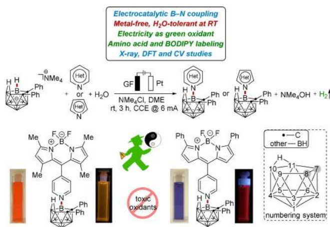
Figure 1. Electrooxidative cage B–H nitrogenation of nido -carborane.
